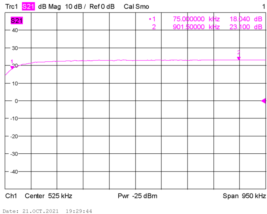
Gain vs Frequency 90kHz-1MHz
